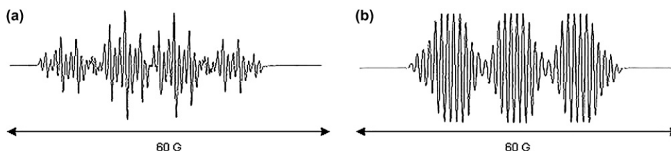
Figure 1. (a) Observed ESR spectrum for the reaction involving equimolar quantities of 3,4-dimethyl-2-( \alpha -[ 2 H]- \alpha -hydroxyethyl)-thiazolium triflate, Et 3 N and PhNO; (b) simulated spectrum of PhND-O \cdot .
