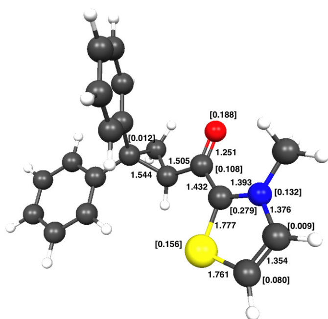
Figure 2. Spin density (ROB3LYP/cc-pVDZ) calculation on radical 6' \leftrightarrow 6'' \leftrightarrow 6''' . Numbers in brackets refer to spin densities.
